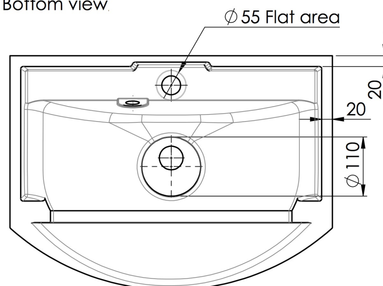
Bottom view
