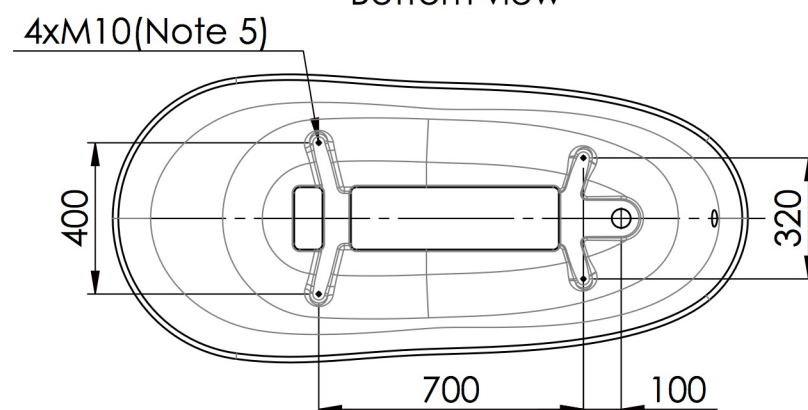
Bottom view
