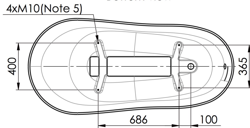
Bottom view
