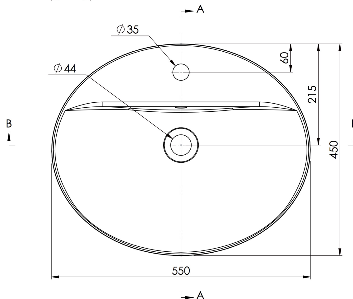
Bottom view
