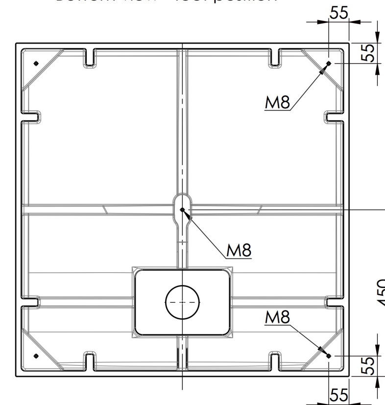
Bottom view - feet position
