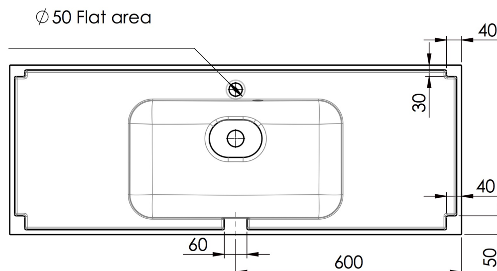
Bottom view
